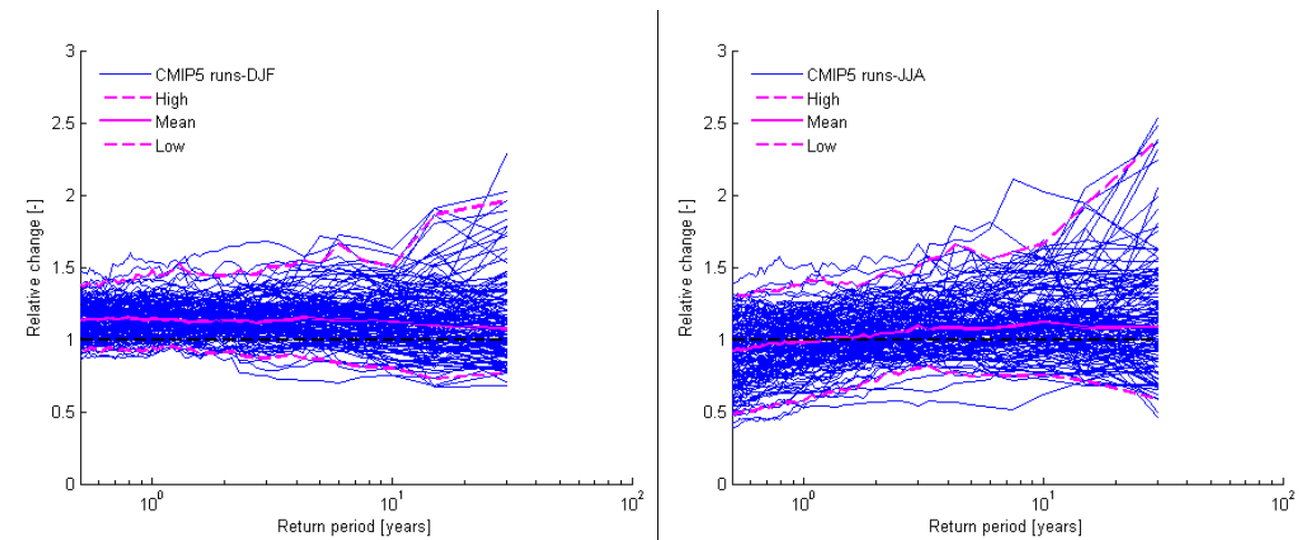
Figure 3.13: Wet day relative change calculated based on control (1961-1990) and scenario (2071-2100) runs versus return periods, for all RCP scenarios and winter season (left) and summer season (right)
