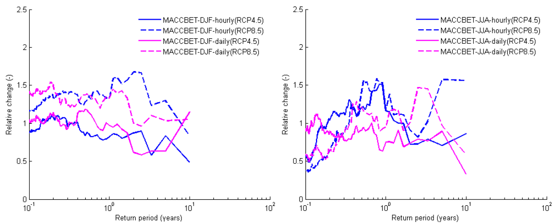
Figure 5.17: Comparison of change factor computed using the MACCBET daily and hourly runs for 2060-2069 horizon and for winter and summer seasons
