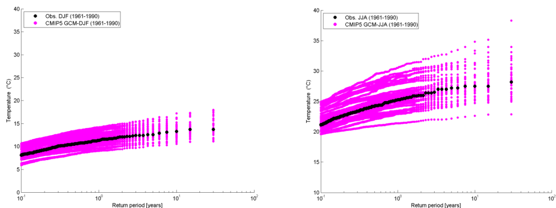
Figure 3.5: Temperature vs. return period: validation of CMIP5 GCM runs based on Uccle historical observations (1961-1990), for winter and summer season
