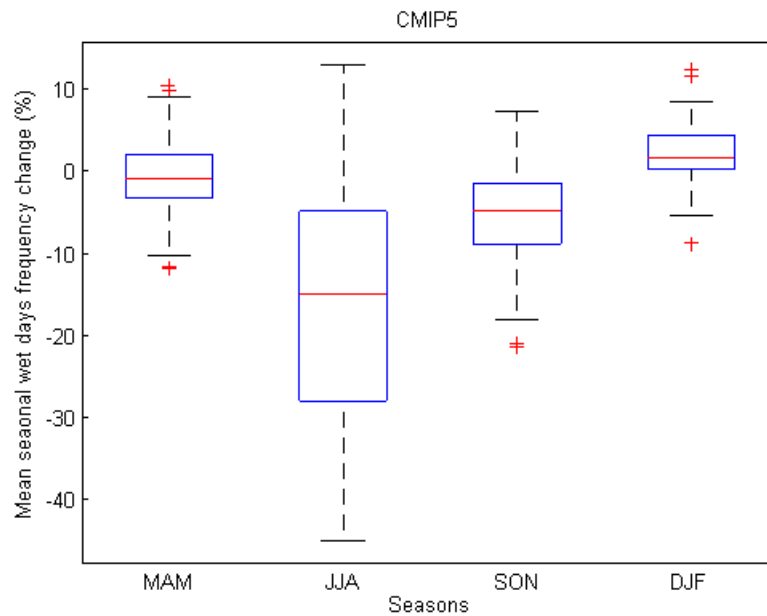
Figure A.1: Mean seasonal number of wet days change summarized for all the seasons based on CMIP5 runs
