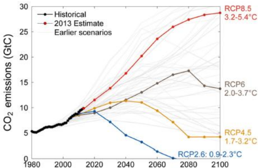
Figure 0.4: Historical versus projected changes in global CO 2 emissions
