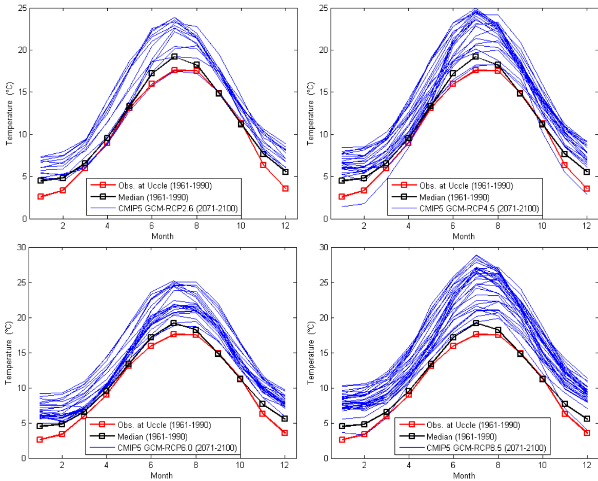
Figure 3.15: Mean monthly temperature for the different CMIP5 GCM future runs (2071-2100), for the individual RCP scenarios, median of control runs (1961-1990) and Uccle observation
