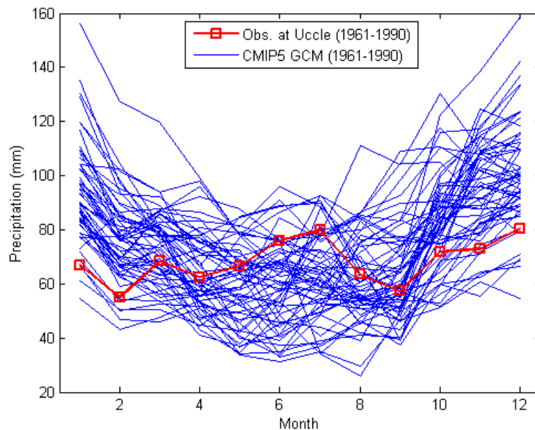
Figure 3.1: Mean monthly precipitation for the different CMIP5 GCM control runs (1961-1990)
