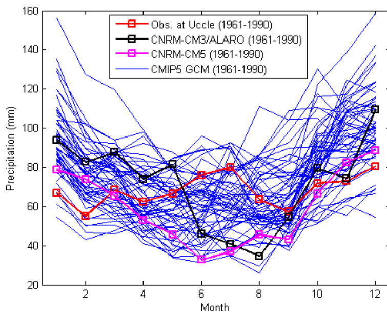
Figure 5.1: Comparison of the CNRM–CM3/ALARO results with the CMIP5 ensemble and Uccle observations, for monthly mean precipitation (historical climate: 1961-1990)
