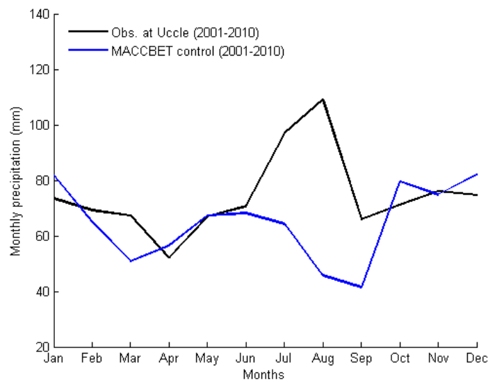
Figure 5.12: Comparison of the MACCBET results with Uccle observations, for monthly mean precipitation (historical climate: 2001-2010)
