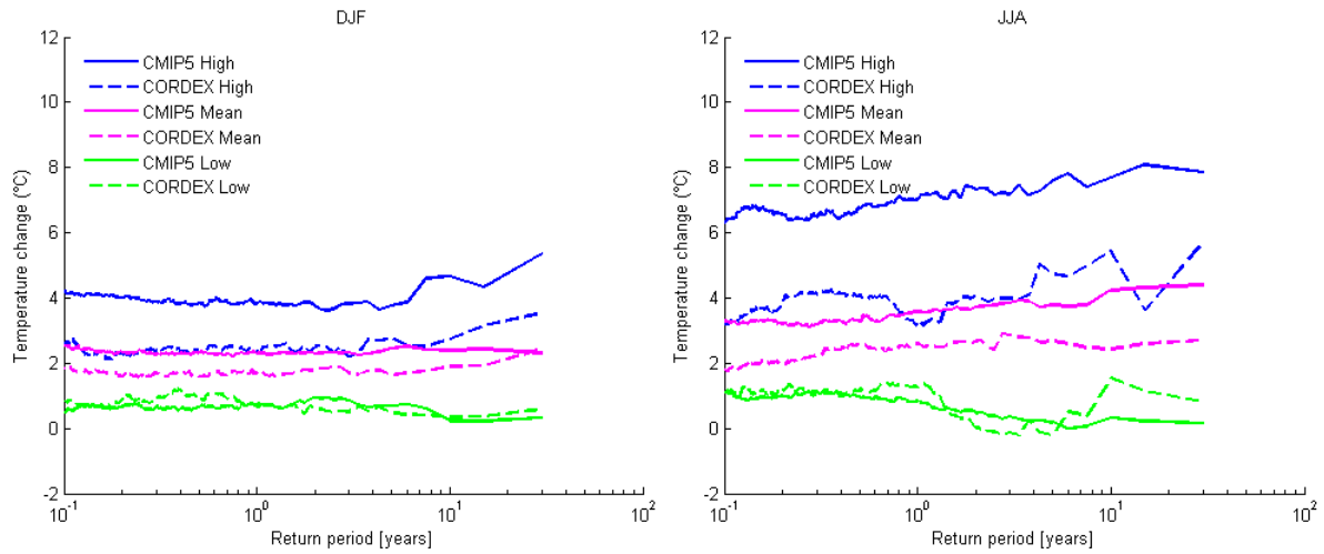
Figure 4.10: High, mean and low relative change values of daily temperature vs. return period: comparison between the CMIP5 GCM runs and CORDEX RCM runs, for winter and summer seasons over 100 years
