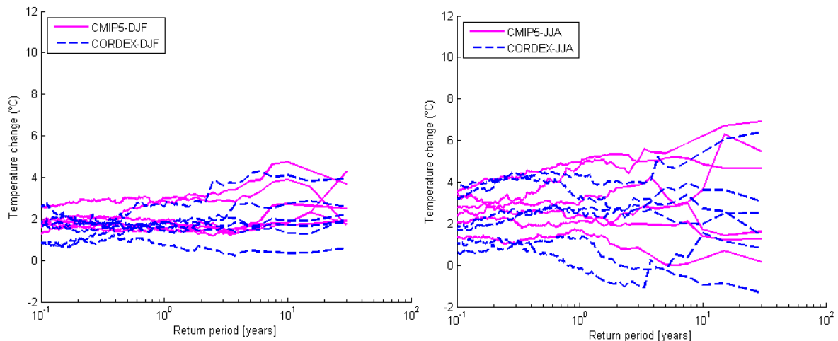
Figure 4.11: Comparison of temperature changes computed using RCP4.5 scenarios of CMIP5 GCM runs and CORDEX runs for winter and summer season
