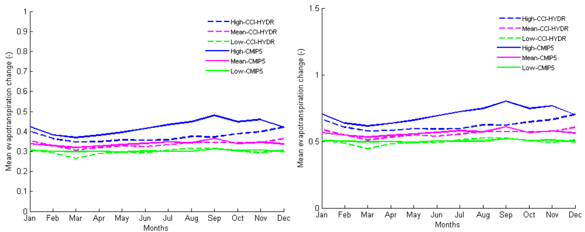
Figure 4.13: High, mean and low scenarios extracted from CMIP5 GCM runs and the CCI-HYDR RCM runs for ETo change factors over 30 years (left) and 50 years (right)
