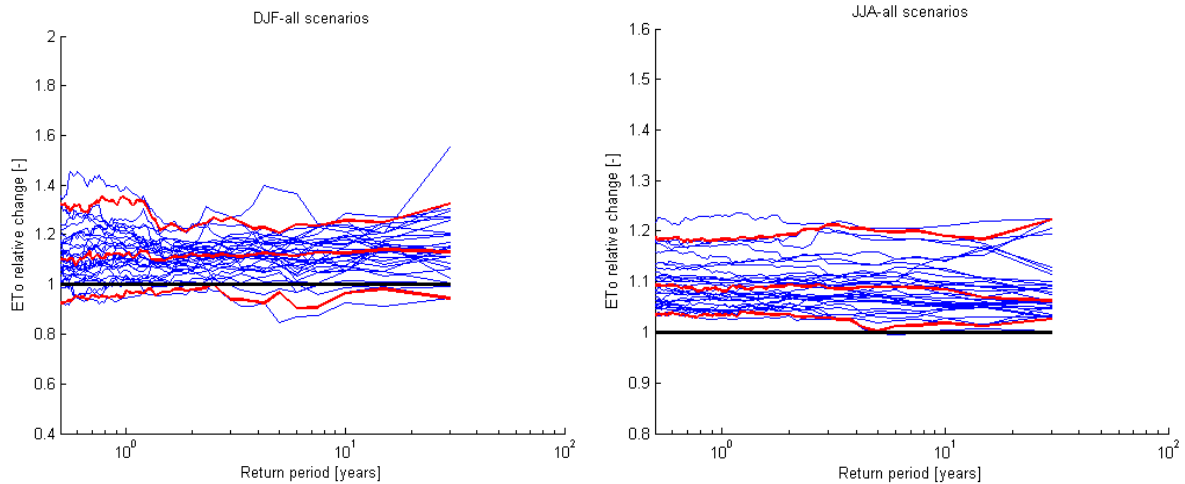
Figure 3.21: ETo change factors vs. return period for the different CMIP5 GCM runs, all RCP scenarios combined, for winter and summer seasons
