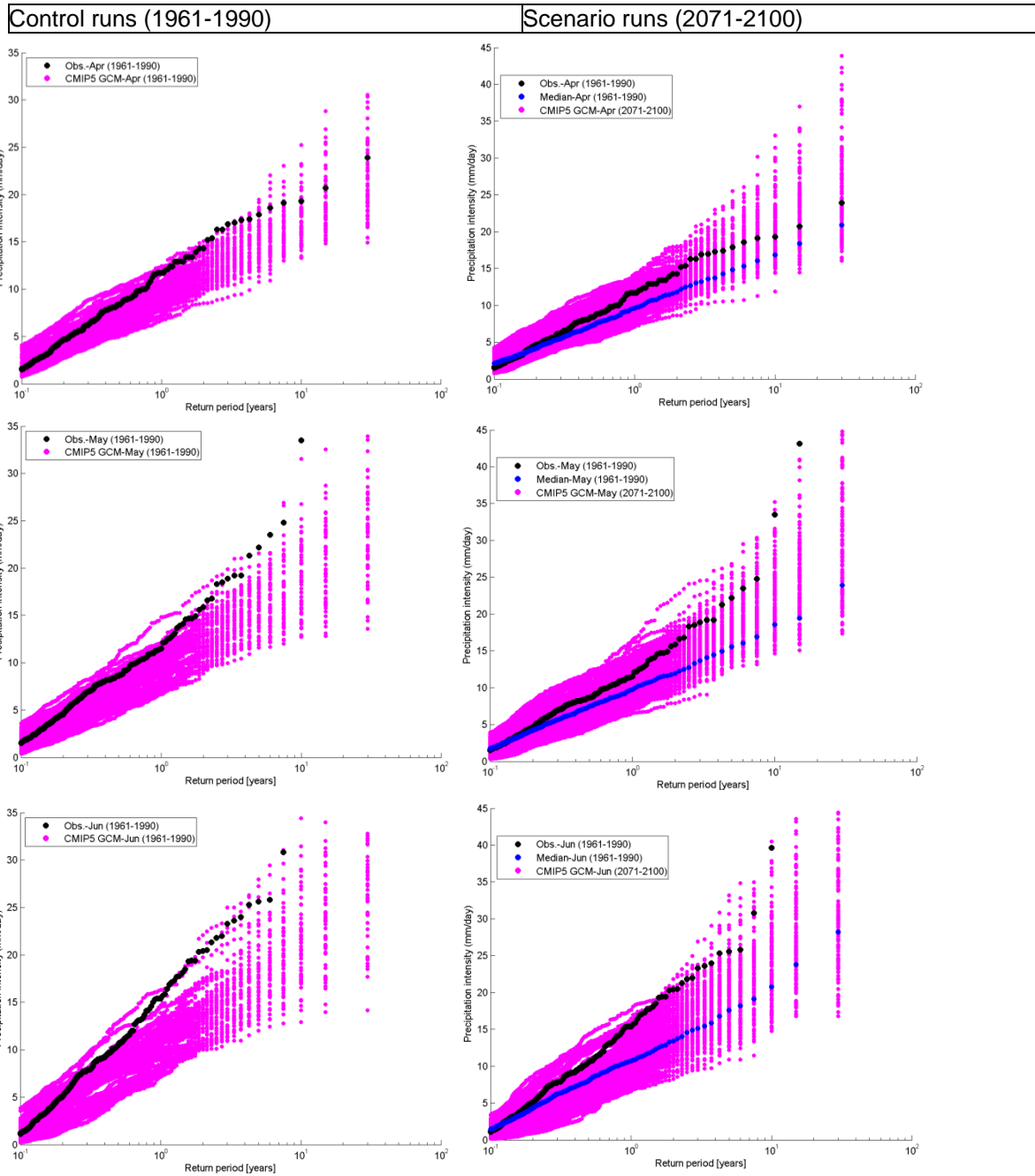
Figure B.2: Wet day precipitation intensities vs. return period: validation of CMIP5 GCM runs based on Uccle historical observations (1961-1990) (left) and comparison with CMIP5 GCM scenario runs (2071-2100) (right), for April to June
