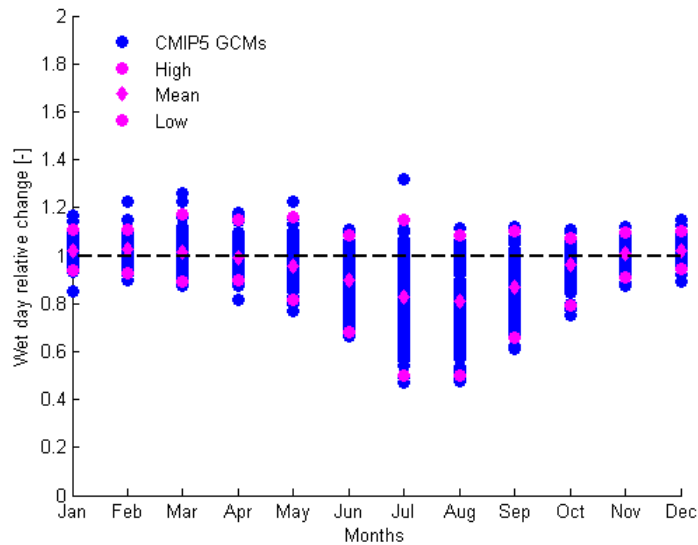
Figure 3.8: Change factors in the number of wet days for all RCP scenarios highlighting high, mean and low scenarios
