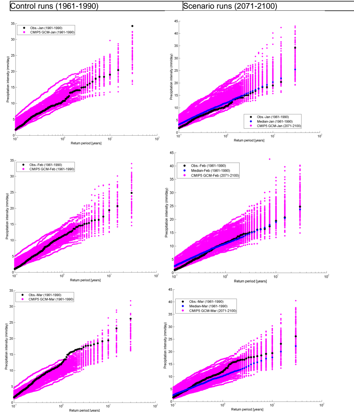
Figure B.1: Wet day precipitation intensities vs. return period: validation of CMIP5 GCM runs based on Uccle historical observations (1961-1990) (left) and comparison with CMIP5 GCM scenario runs (2071-2100) (right), for January to March
