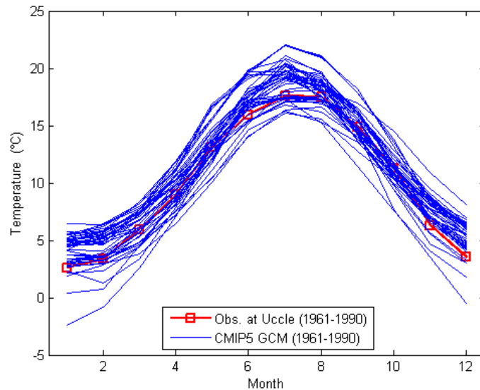
Figure 3.4: Mean monthly temperature for the different CMIP5 GCM control runs (1961-1990)
