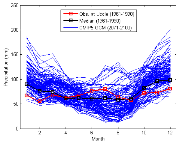
Figure 3.9: Mean monthly precipitation for the different CMIP5 GCM future runs (2071-2100), for combined RCP scenarios, median of control runs (1961-1990) and Uccle observation
