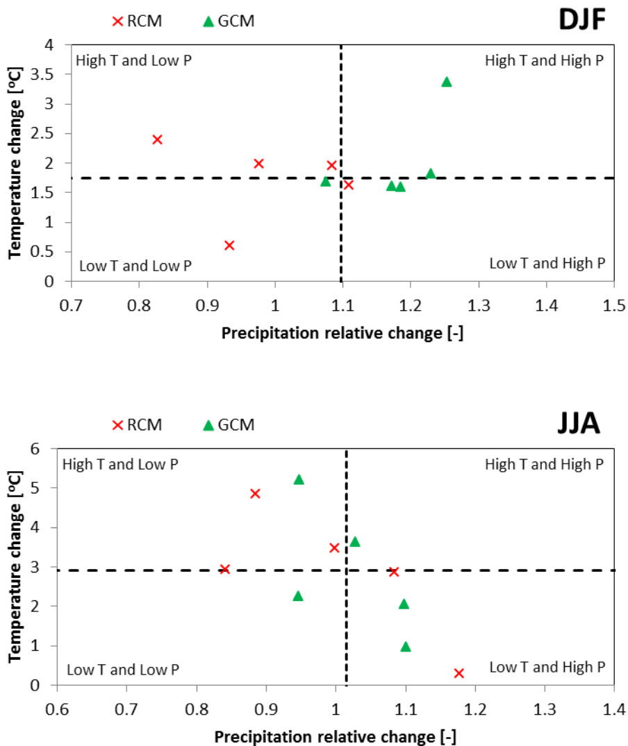
Figure 4.22: Inter-seasonal tracing of precipitation and temperature relative changes (averaged for return periods >1 year, over 100 years) for CORDEX and GCM scenarios
