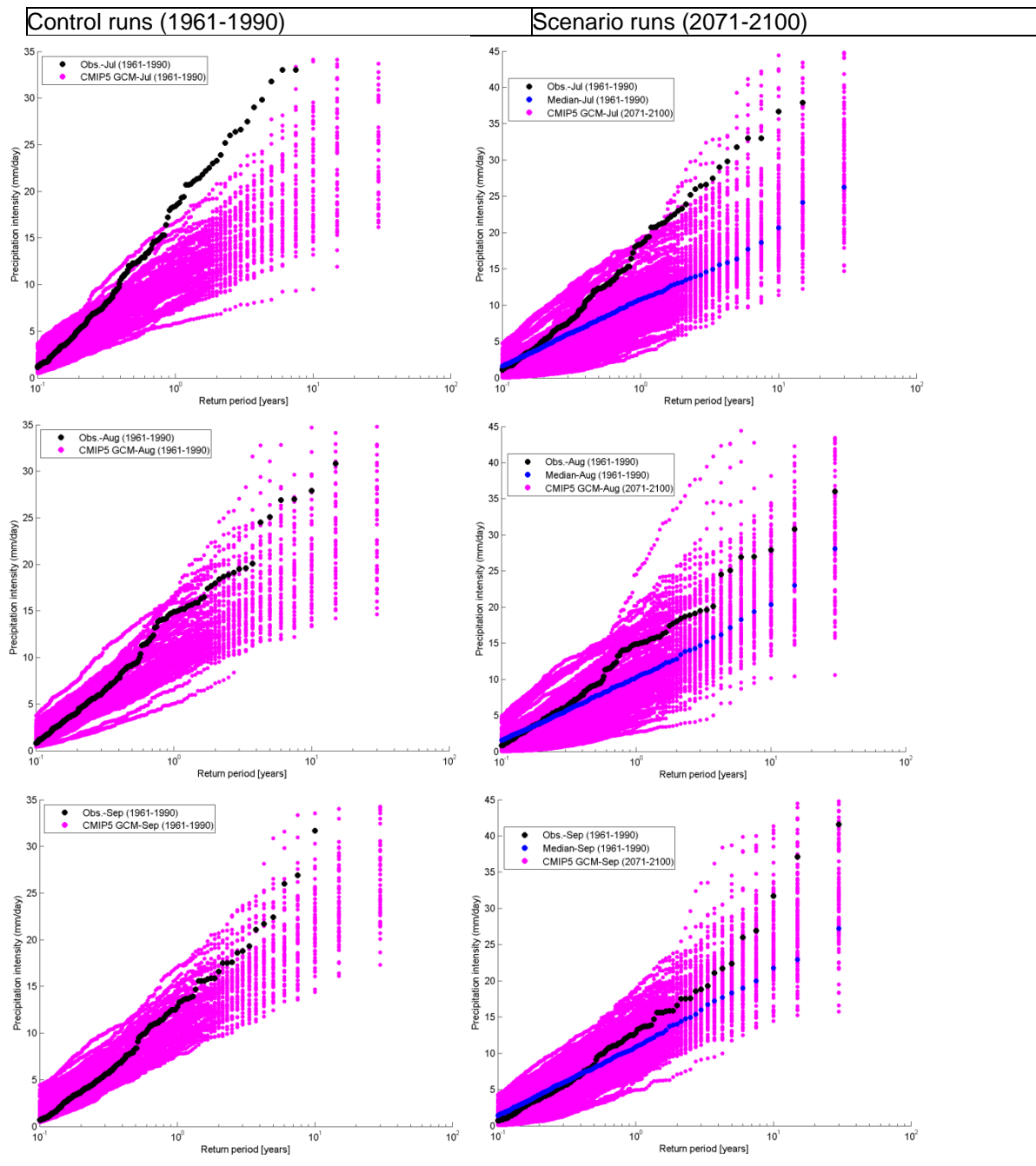
Figure B.3: Wet day precipitation intensities vs. return period: validation of CMIP5 GCM runs based on Uccle historical observations (1961-1990) (left) and comparison with CMIP5 GCM scenario runs (2071-2100) (right), for July to September
