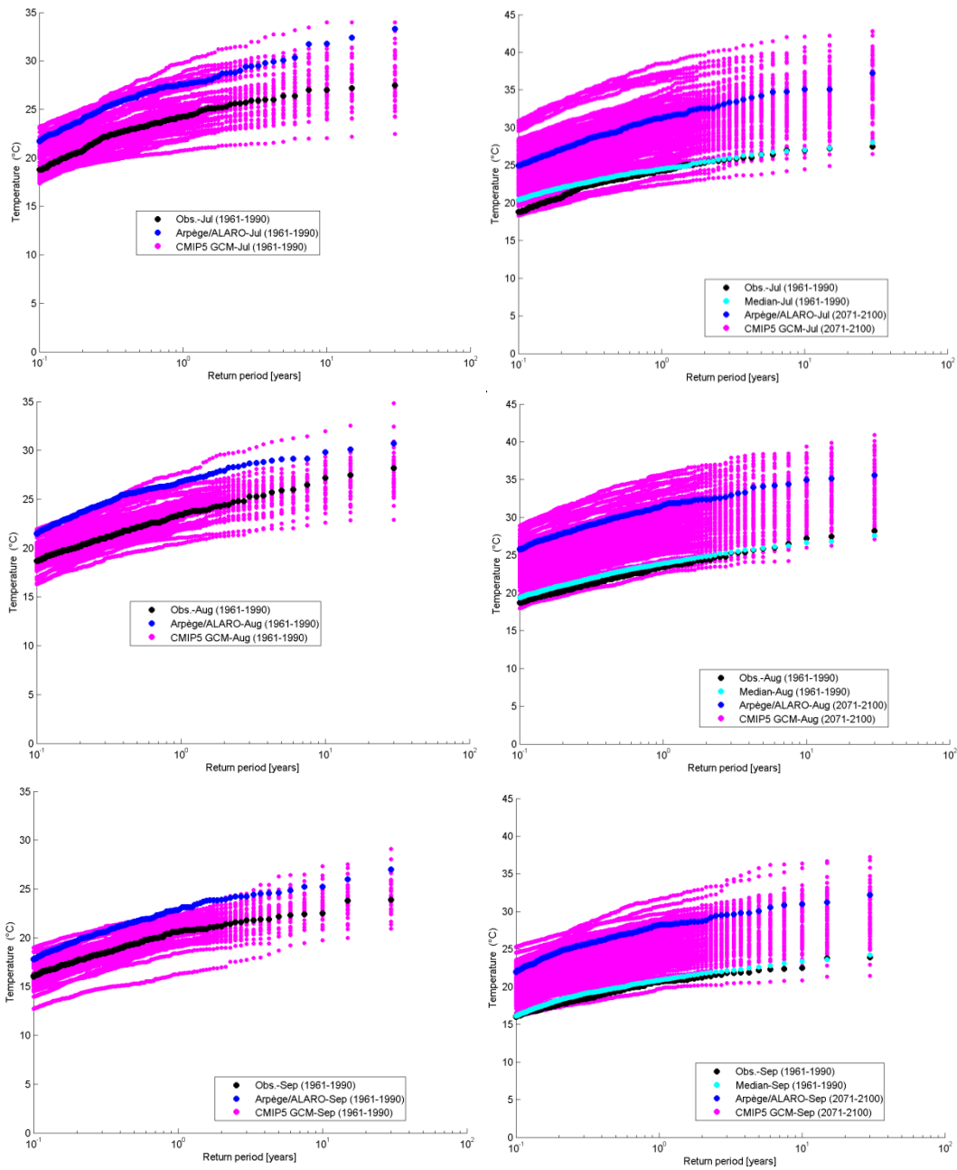
Figure B.10: Temperature vs. return period: comparison of control and scenario period runs for months July to September
